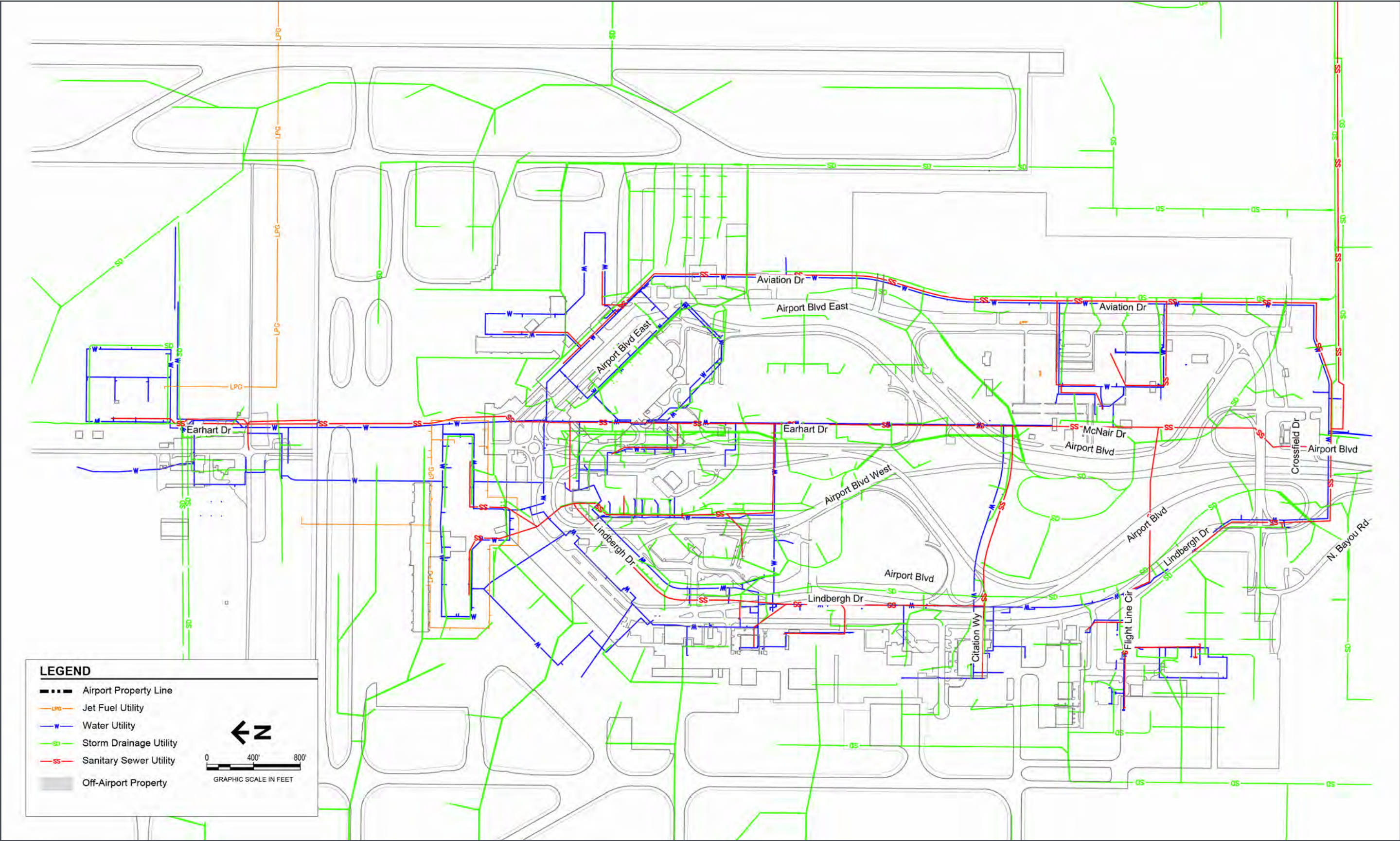
Figure 1-20 Wet Utilities
